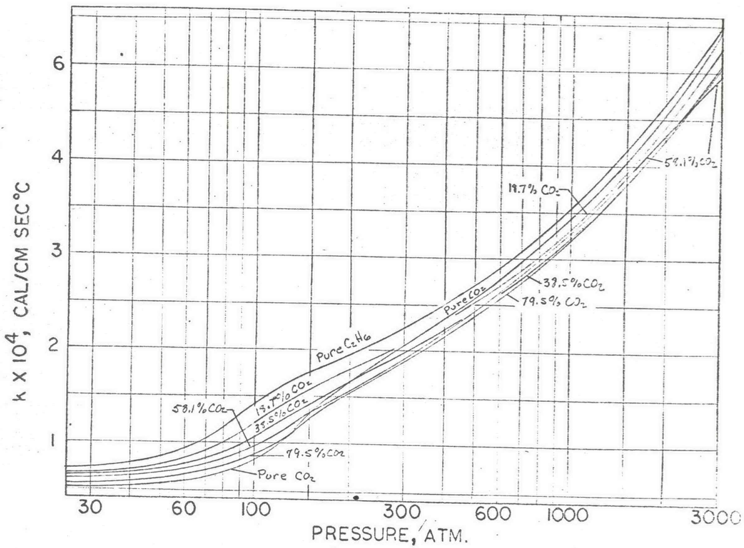
FIGURE 7. THERMAL CONDUCTIVITY OF CO 2 -C 2 H 6 MIXTURES AT 75°C
